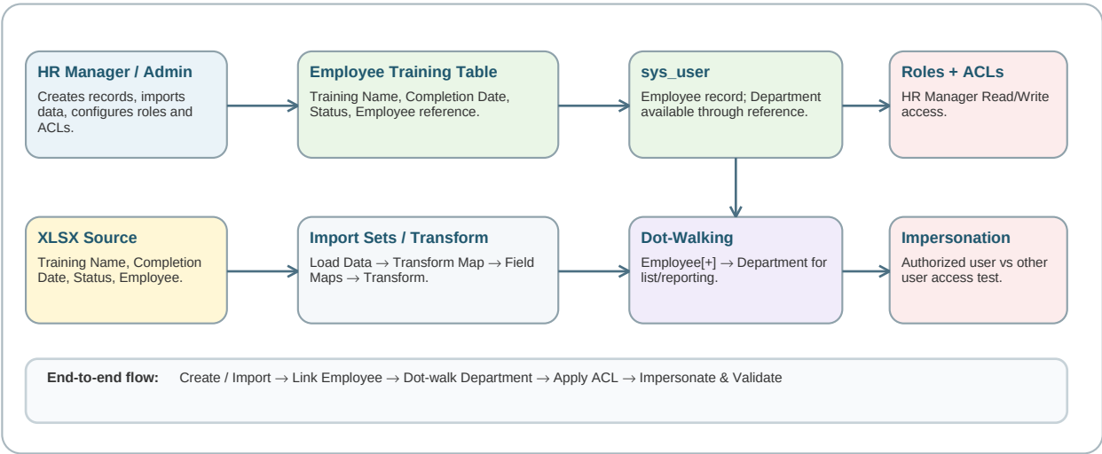
Figure 1: Solution architecture and data flow of the ServiceNow Employee Training Access Control solution
